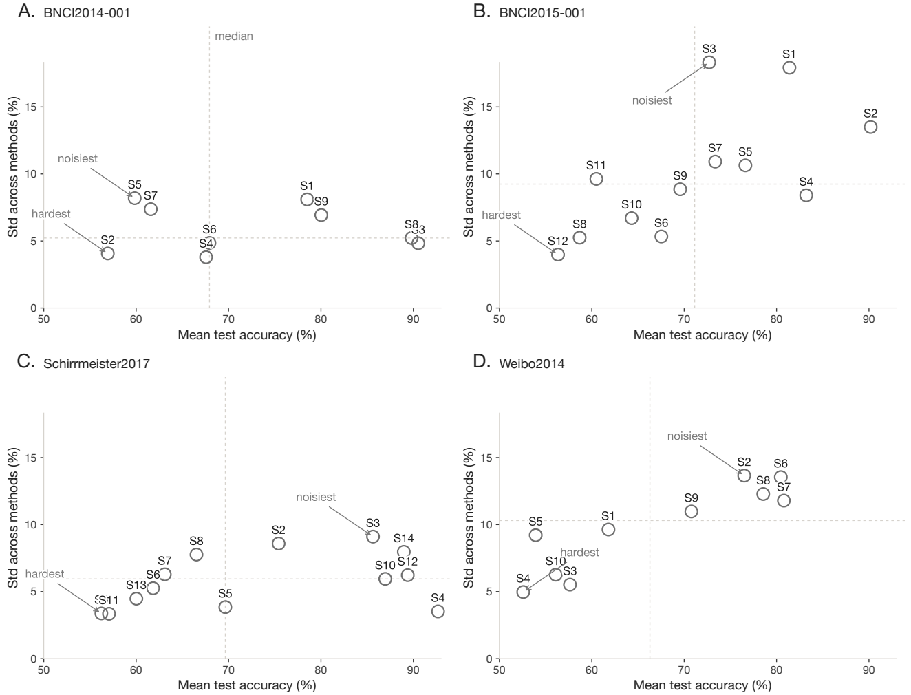
Figure 12. Subjects split into a consistently-hard mode and a method-noisy mode, with the mix changing per dataset. Each point is one subject; x = mean test accuracy across all 18 method \times alignment \times head-selection combinations; y = standard deviation of that same population. Dashed grey lines mark per-panel medians; the resulting quadrants read as: lower-left = consistently hard, lower-right = consistently easy, upper-half = method-noisy. The callouts label the lowest-mean and highest-std subjects per dataset. Subject behaviour is heterogeneous and at least two-dimensional: method-noisy subjects sit anywhere along x , including near-ceiling accuracy.
