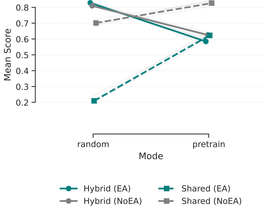
Figure 10. Subject identity persists after training but evolves oppositely across architectures. Linear subject-identity decoding accuracy from EEGNet encoder features on the BNCI2014 dataset, evaluated at random initialization (left) and after training (right), for the hybrid encoder bank and the shared encoder, with and without Euclidean Alignment (EA). Each line tracks one architecture/alignment combination from its random-init score to its trained score. The hybrid encoder loses subject identifiability with training regardless of EA, converging from \sim 0.80 to \sim 0.60 under both conditions. The shared encoder shows the opposite trend and is markedly EA-dependent: under EA it starts near floor ( \sim 0.20 ) and rises sharply after training ( \sim 0.67 ), while without EA it starts already substantial ( \sim 0.7 ) and rises more modestly ( \sim 0.82 ).
