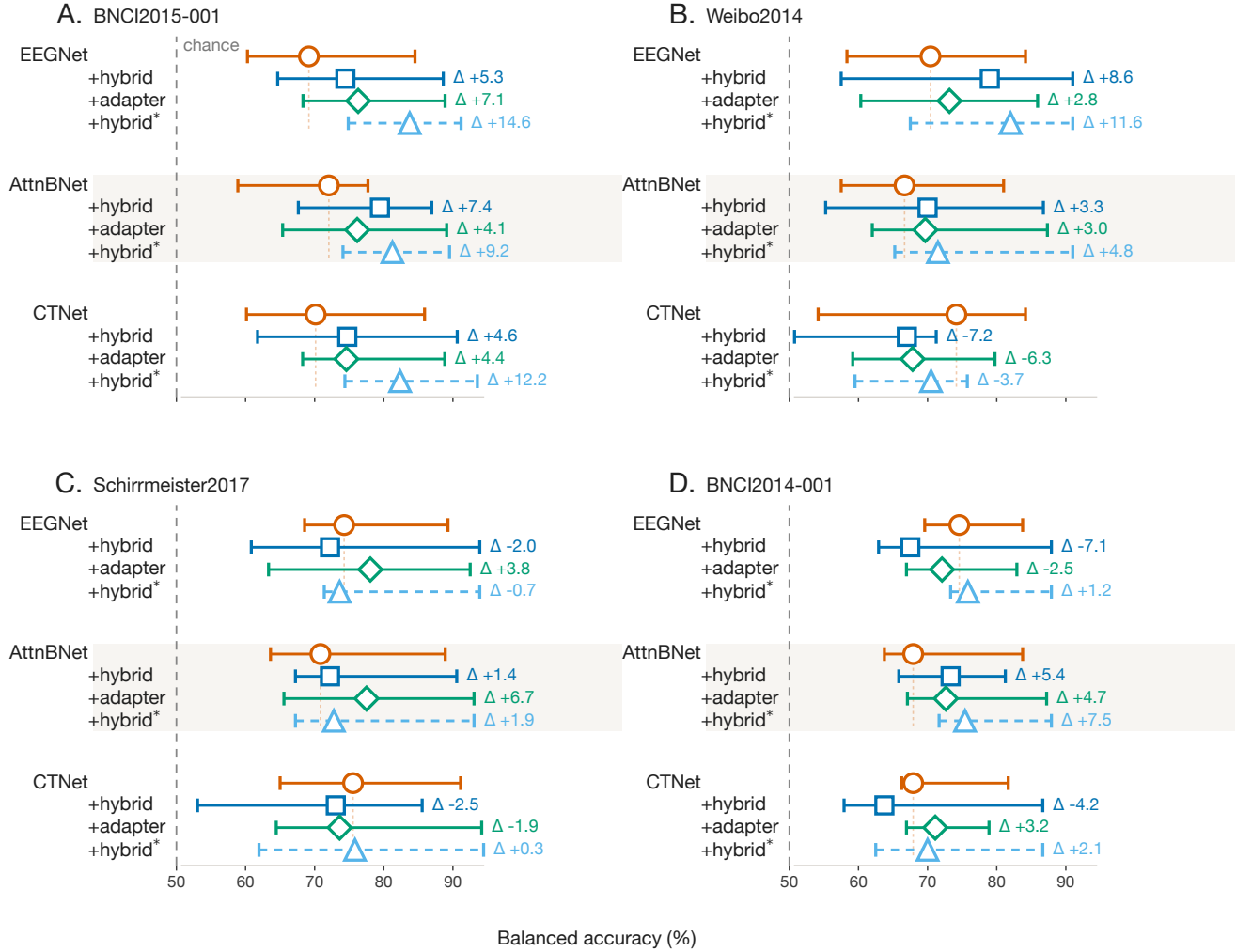
Figure 5. Per-subject balanced accuracy of the proposed +hybrid extension, a low-rank per-subject adapter (+adapter), and the oracle ceiling +hybrid*, compared to plain baselines, across three backbones (EEGNet, AttnBNet, CTNet) on four motor-imagery datasets under Euclidean Alignment. Open markers give the subject median; horizontal bars span the inter-quartile range; the dashed line marks chance accuracy. Within each backbone block the rows are, top to bottom, the plain baseline (vermillion circle), the full per-subject encoder +hybrid (blue square), the rank-2 low-rank adapter +adapter (green diamond), and the oracle +hybrid* (light-blue triangle). The adapter is deployable and calibration-selected like +hybrid, differing only in the per-subject module. The thin vermillion vertical guide marks that block’s plain-baseline EA median; the \Delta annotation on each +hybrid, +adapter, and +hybrid* row reports median balanced accuracy minus that baseline median, both measured under EA. The oracle variant selects each subject’s best test-set head and therefore serves only as an upper bound for any validation-based head selection. Datasets are arranged in reading order (top-left to bottom-right) by the average +hybrid – baseline gap across the three backbones, so the largest hybrid wins appear in the top-left panel.
